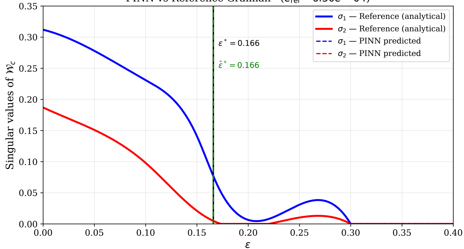
PINN vs Reference Gramian ( e_{\text{rel}} = 6.30e - 04 )
